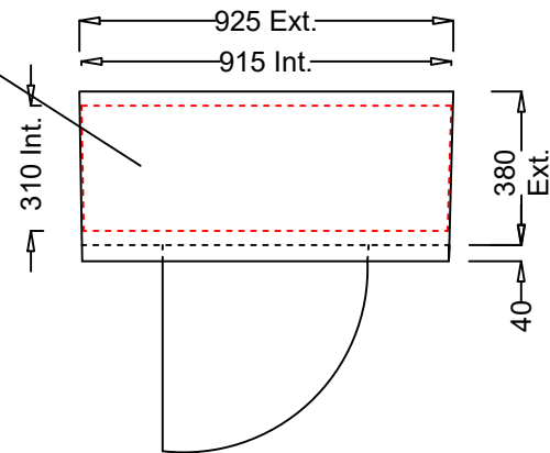
Non Load bearing GRP Floor
